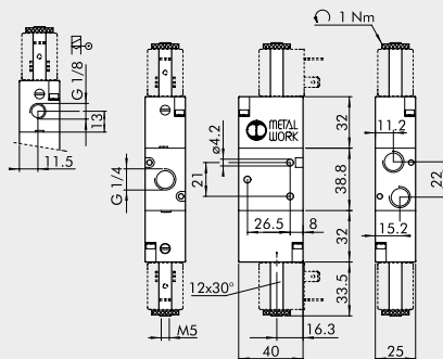
BISTABLE 3/2, 1/4"
