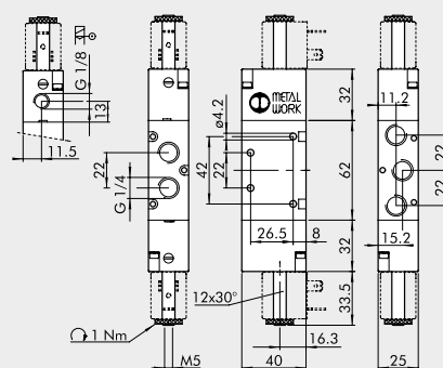
DOUBLE 3/2, 1/4"
